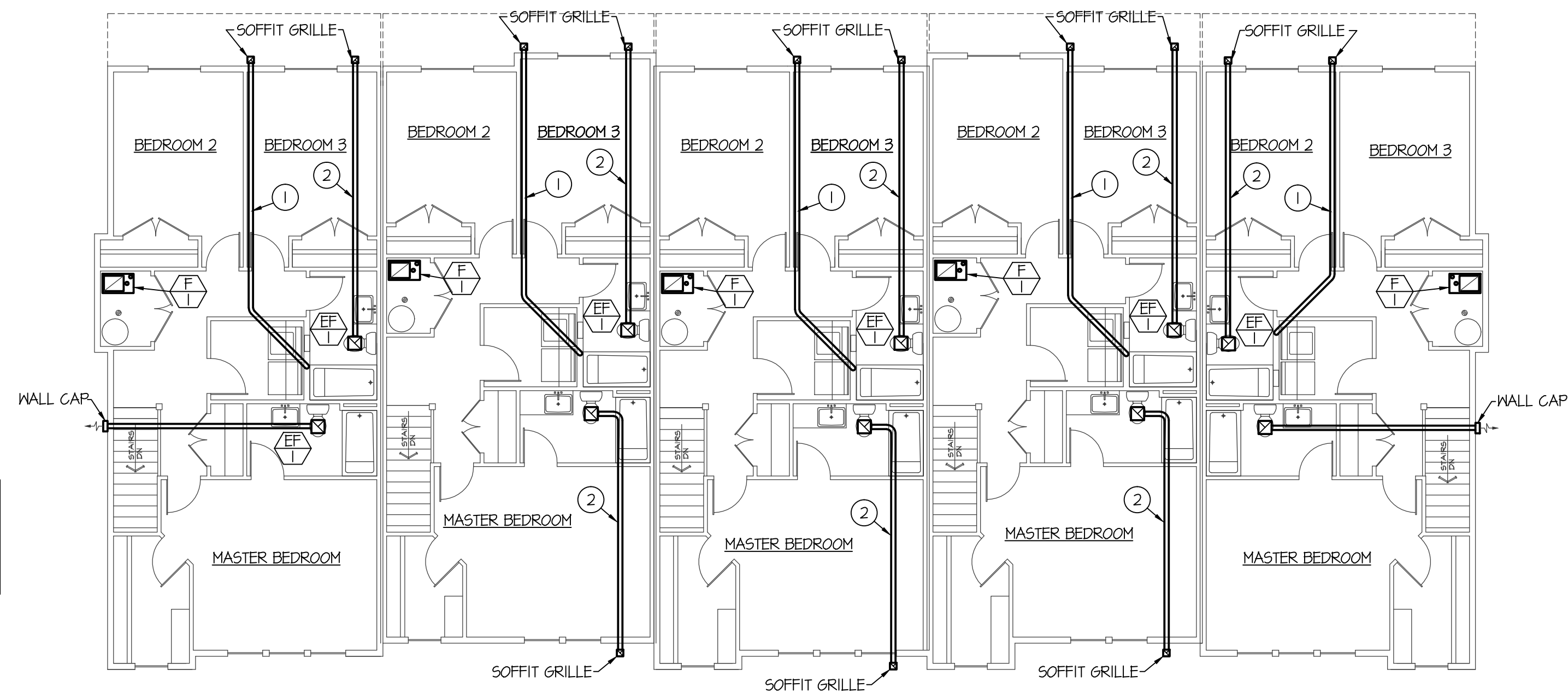
BUILDING "A" UPPER LEVEL MECHANICAL PLAN SCALE: 1/8" = 1'-0"
