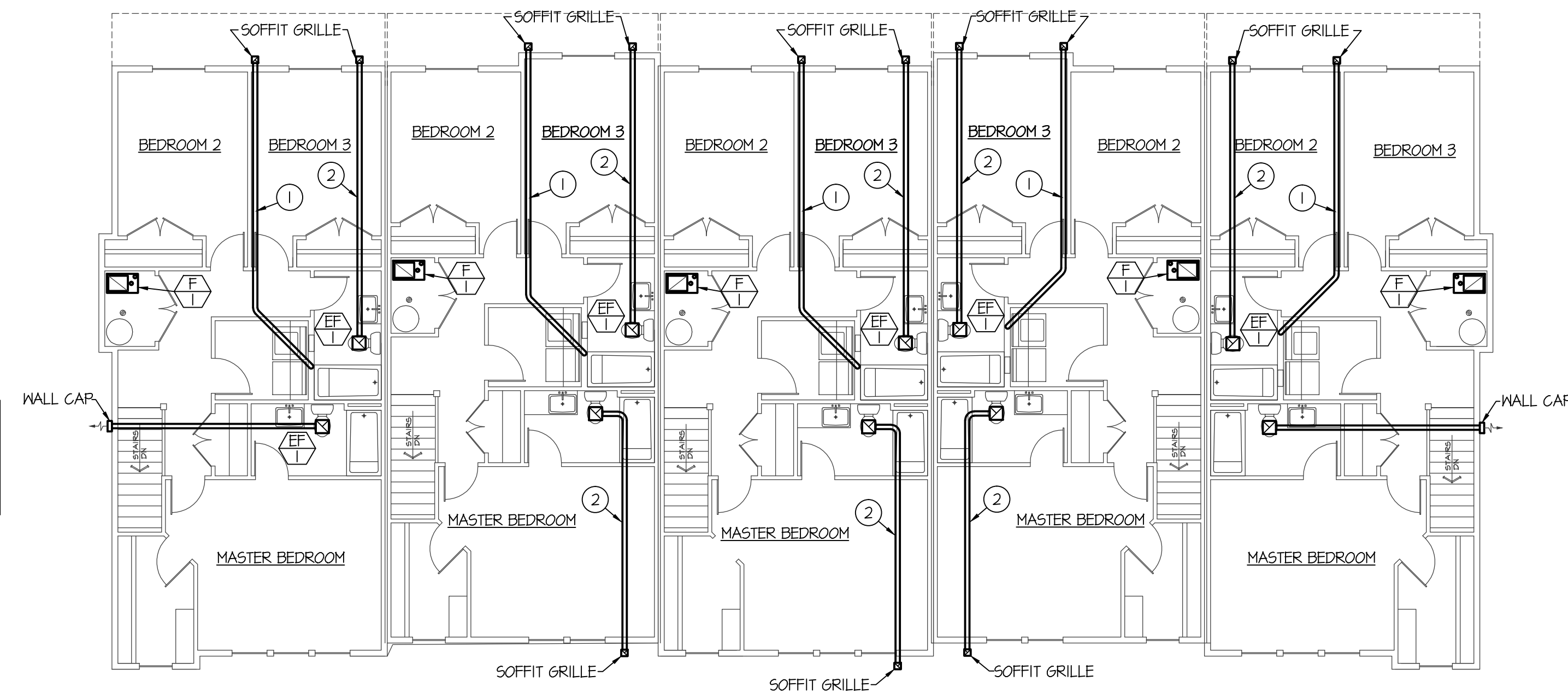
BUILDING "B" UPPER LEVEL MECHANICAL PLAN SCALE: 1/8" = 1'-0"
